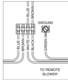
Remote blower wiring.
