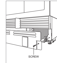
Kickplate removal
