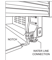
Water line
