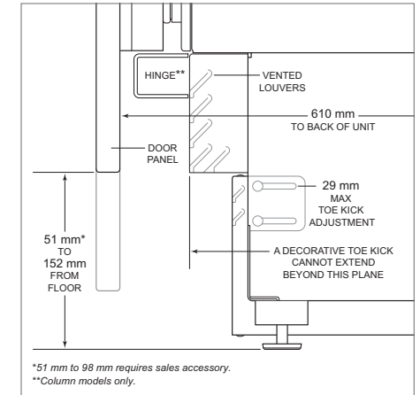
Toe kick (side view)
