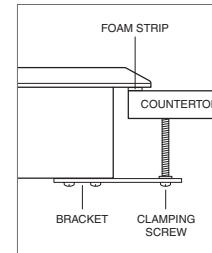
Cooktop installation
